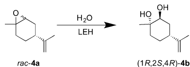
Scheme 3. Hydrolysis of limonene epoxide rac - 4a by LEH.
